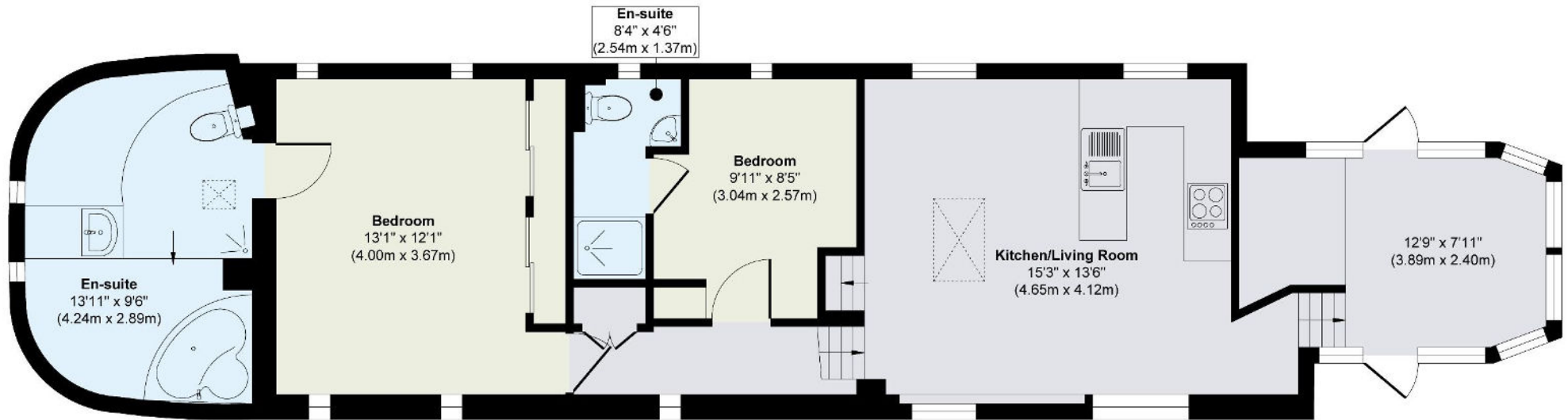
Floor Plan
